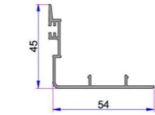
Alm. Kanat Arka Kapama 16051.601.5.1.1.9016
