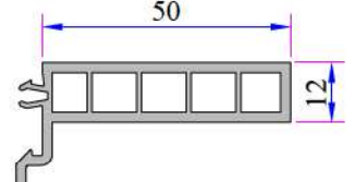
Kasa Pervaz Profili (50mm) 099.5524
